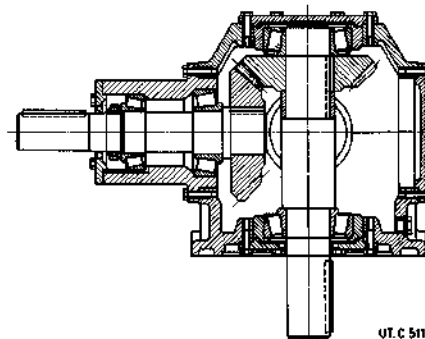
albero lento normale standard low speed shaft
