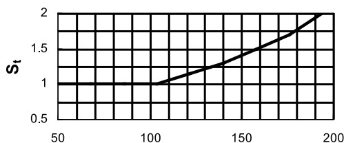
Figure 1: Temperature Factor*, S_t (HTR)
