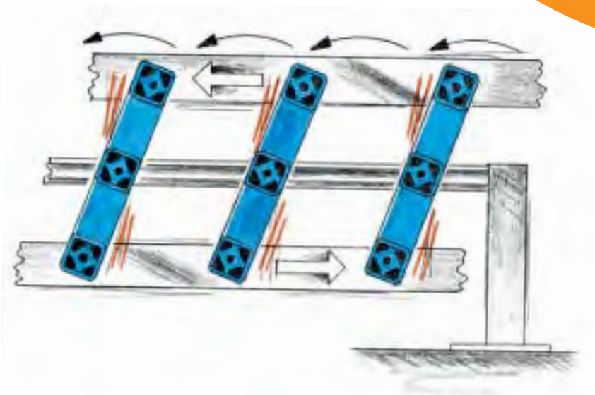
Double rocker arms for high speed shaker conveyors
