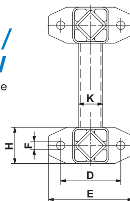
Type AS-PV with inverted flange
