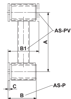
Type AS-PV with inverted flange
