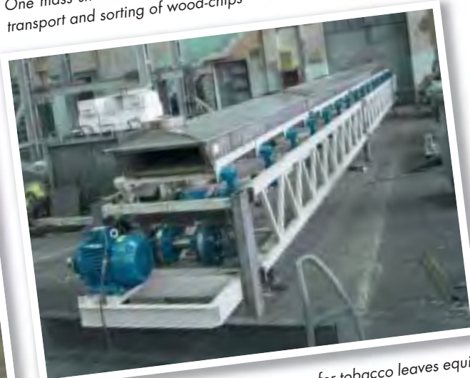
Stainless steel rocker arms in welded construction supporting a foodstuff shaker conveyor
